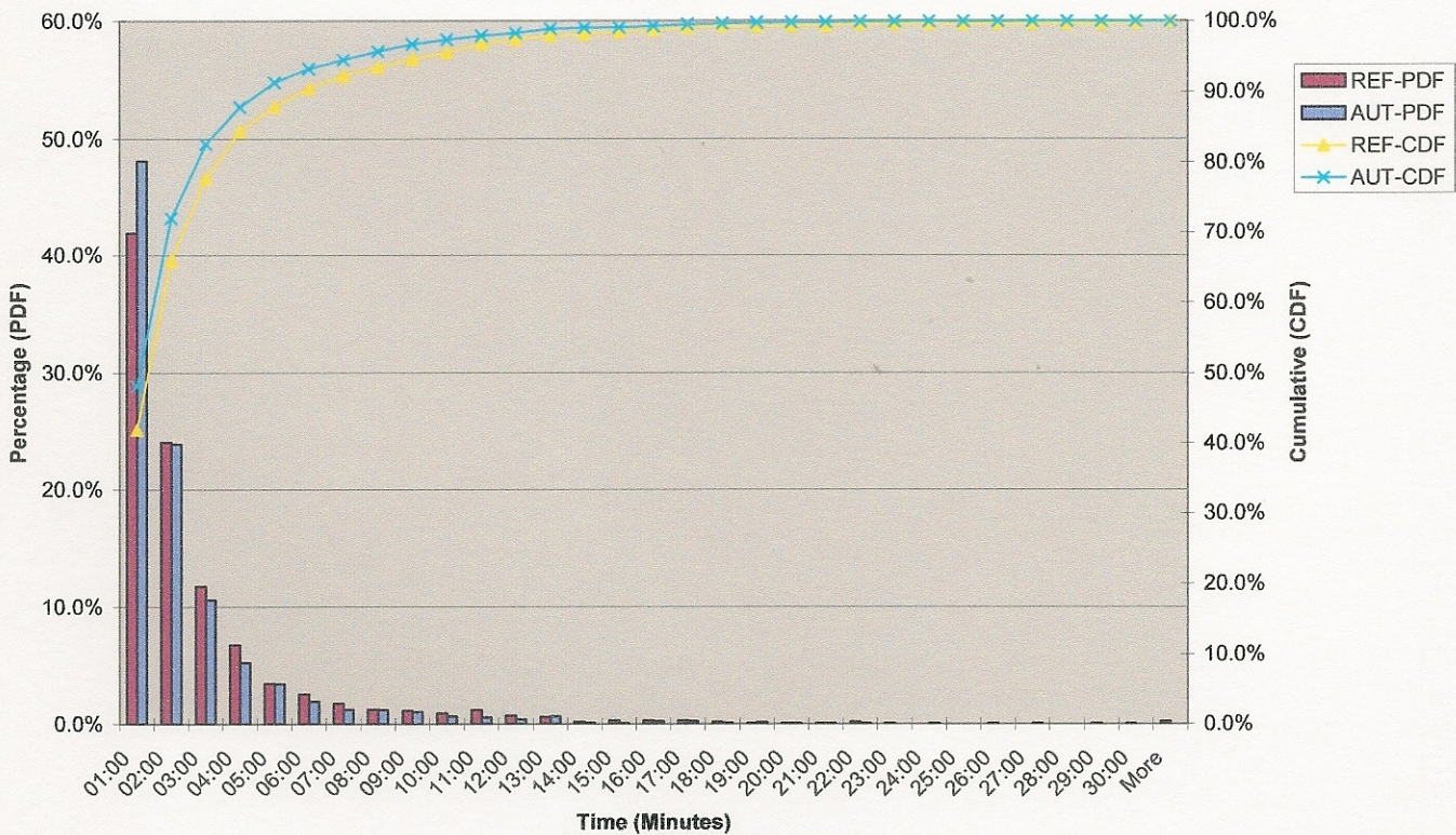
100 Byte Message Test Inevitable Technologies 1/4 Wave vs Reference Half Wave Total Msgs: 2169 vs 1760 Msgs/Hr 30 vs 24
